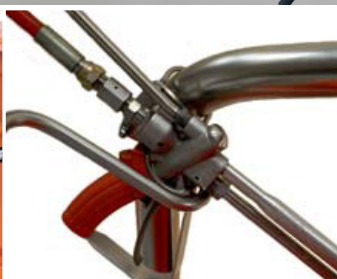
Stainless steel top-frame with gun rest / lance holder.
