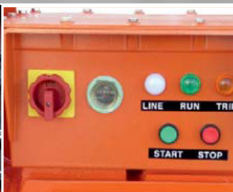
Die cast electrical box with main switch, overload relay & hour meter.
